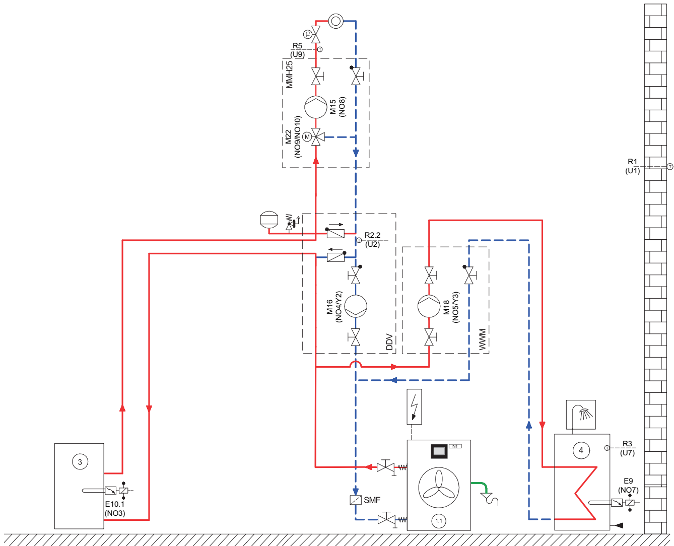
hydraulic 2
