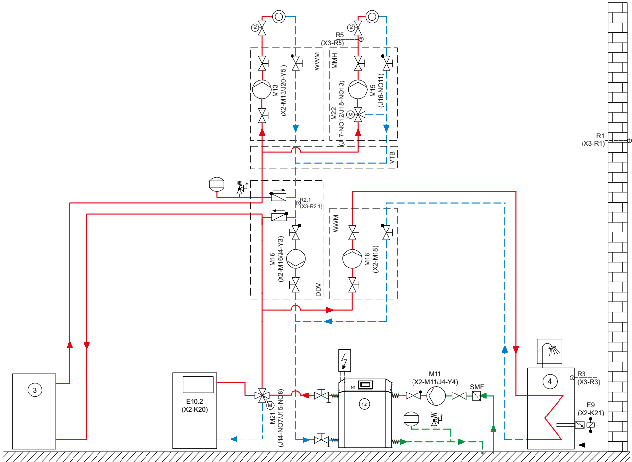
hydraulic 1
