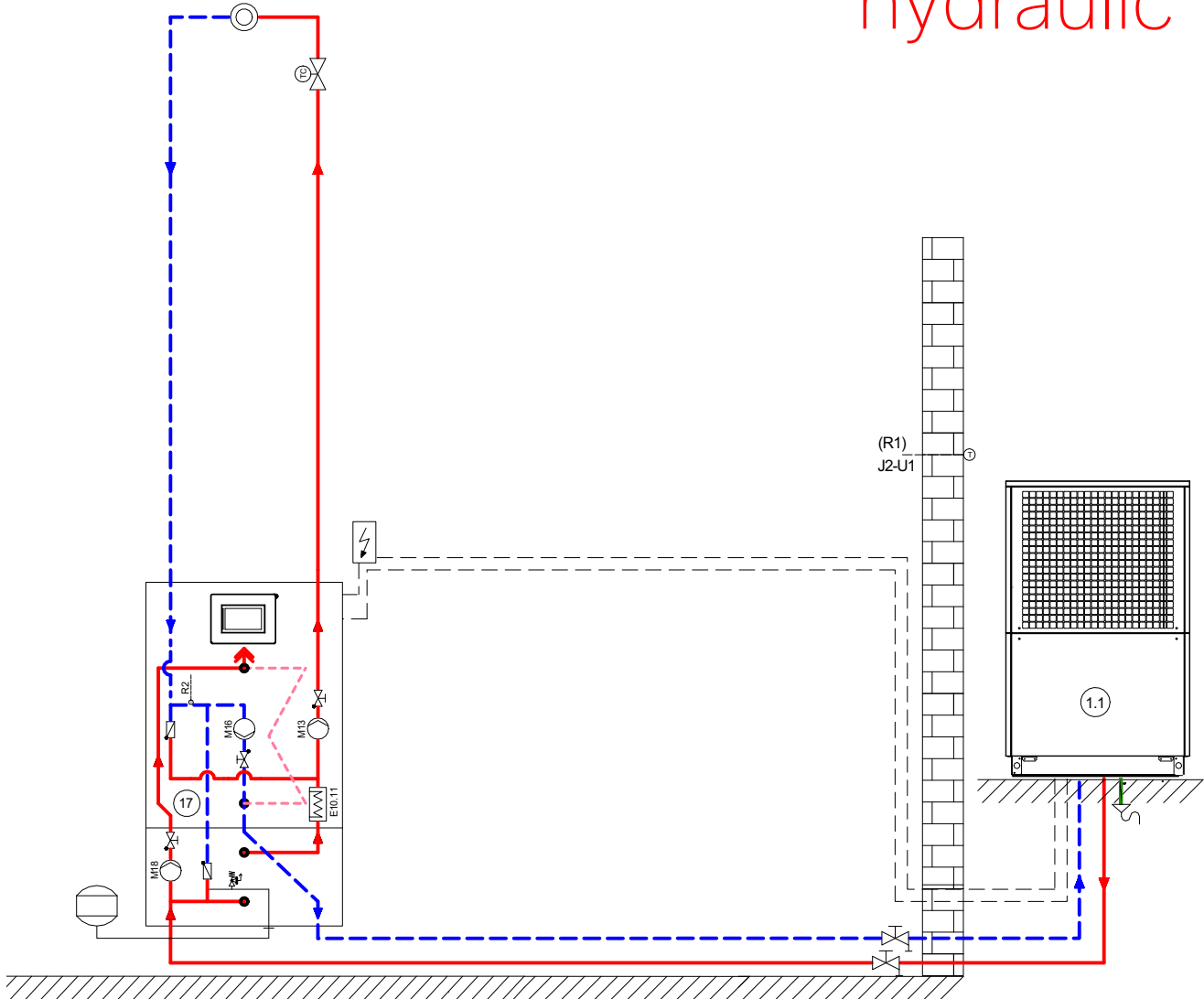
hydraulic 1
